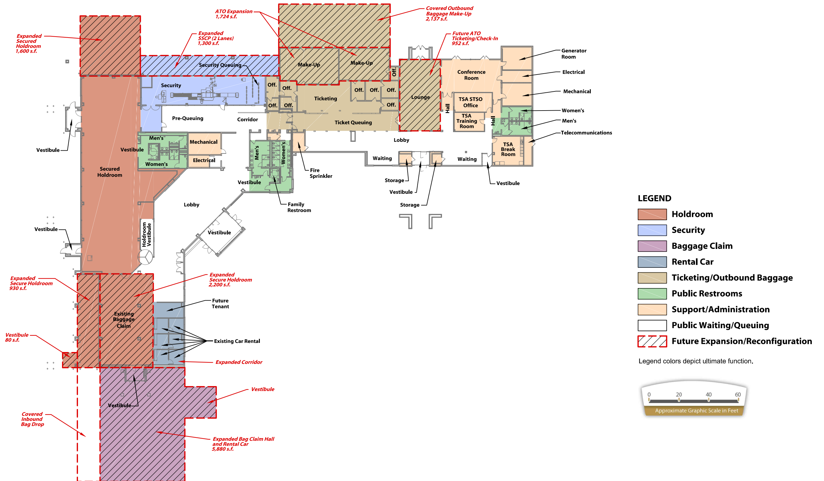
FIGURE D3 Terminal Building Expansion Options
